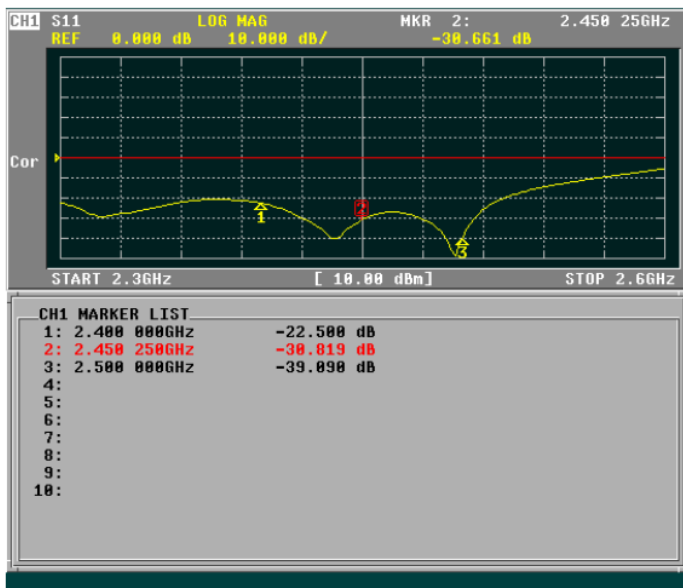
Return loss
