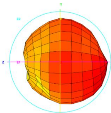
Total_3D_Left View_878MHz
