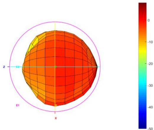
Total_3D_Left View_868MHz
