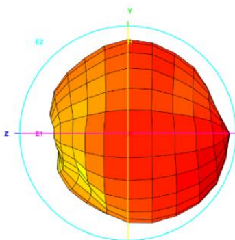
Total_3D_Left View_868MHz
