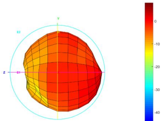
Total_3D_Left View_868MHz
