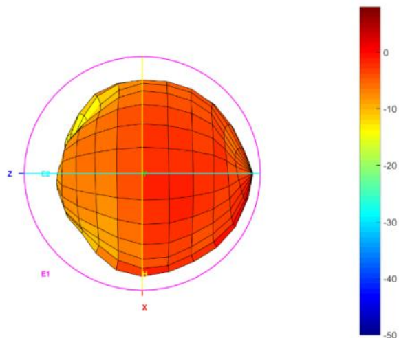
Total_3D_Left View_878MHz
