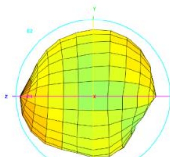
Total_3D_Left View_428MHz
