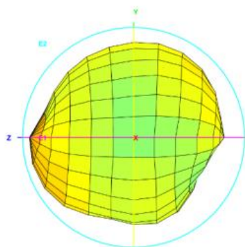
Total_3D_Left View_433MHz
