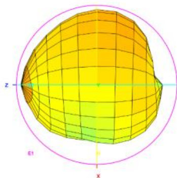
Total_3D_Left View_428MHz
