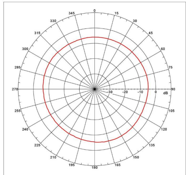
Far-field amplitude for 1 800 MHz
