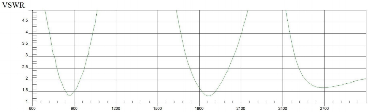
VSWR AO-AGSM-TG09
