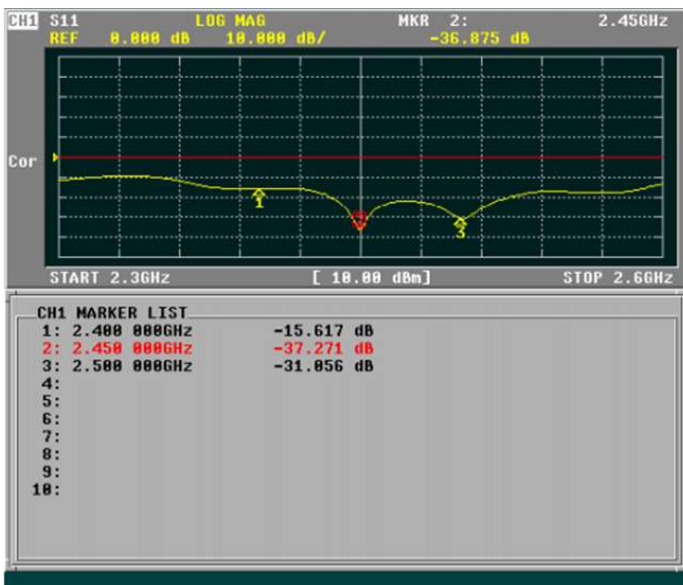
Return loss
