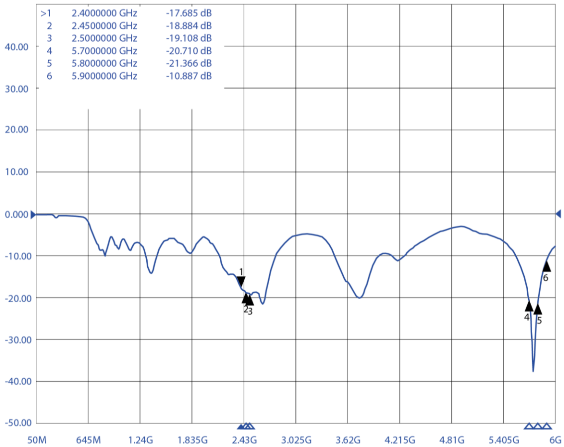
Tr1 S11 Log Mag 10.00dB/REF 0.000dB
