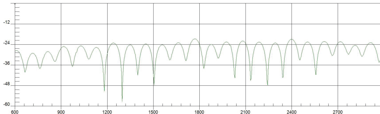
GRAPH S12 - RETURN LOSS [dB]
